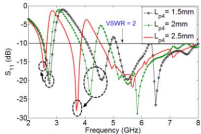
Fig. 5. Simulated magnitude of S_{11} of the proposed antenna for various L_{p4} at L_{p1} = 6.5 mm.
