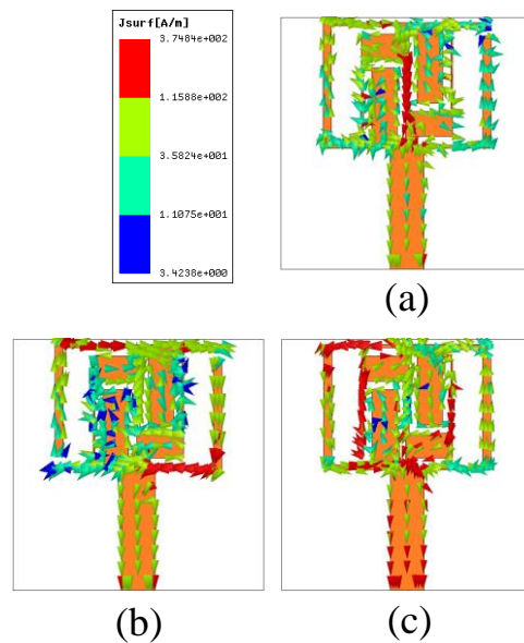
Fig. 8. Surface current distribution on the patch antenna at various resonance frequencies, (a) 2.54 GHz, (b) 3.7 GHz, and (c) 5.8 GHz.
