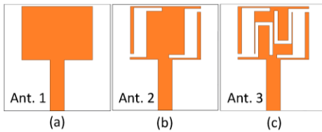
Fig. 2. Configuration of antennas with (a) an ordinary patch (Ant. 1), (b) a pair of symmetrical L- shaped slots on the patch (Ant. 2) and (c) a pair of symmetrical L- and U- shaped slots (Ant. 3).
