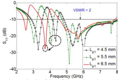
Fig. 4. Simulated magnitude of S_{11} of the proposed antenna for various L_{p1} at L_{p4} = 2.5 mm.
