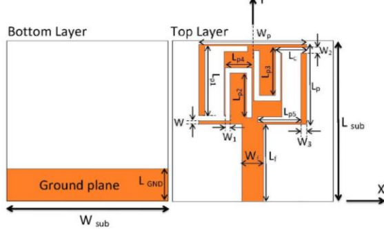
Fig. 1. Configuration of the proposed antenna.
