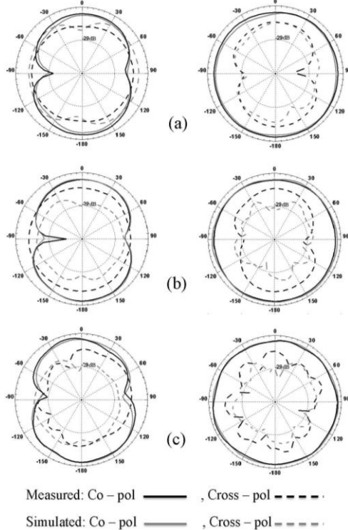
Fig.10. The measured and simulated (left) E - plane and (right) H - plane radiation patterns of the proposed antenna at: (a) 2.54 GHz, (b) 3.7 GHz, and (c) 5.65 GHz.
