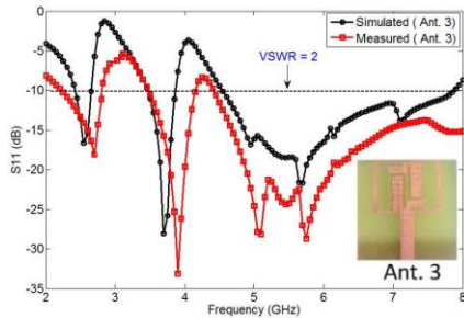
Fig. 9. Measured and simulated magnitude of S_{11} for Ant. 3.
